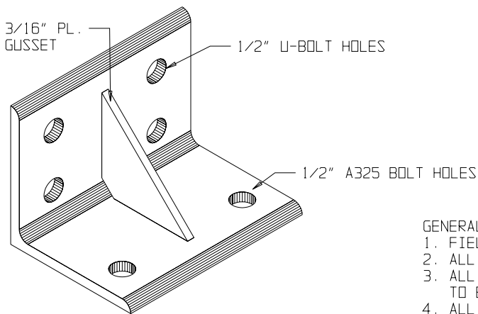
ANGLE MOUNTING BRACKET L3.5x3.5x1/4
